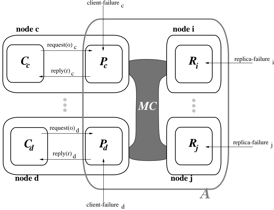
Figure 1: Implementation Architecture
