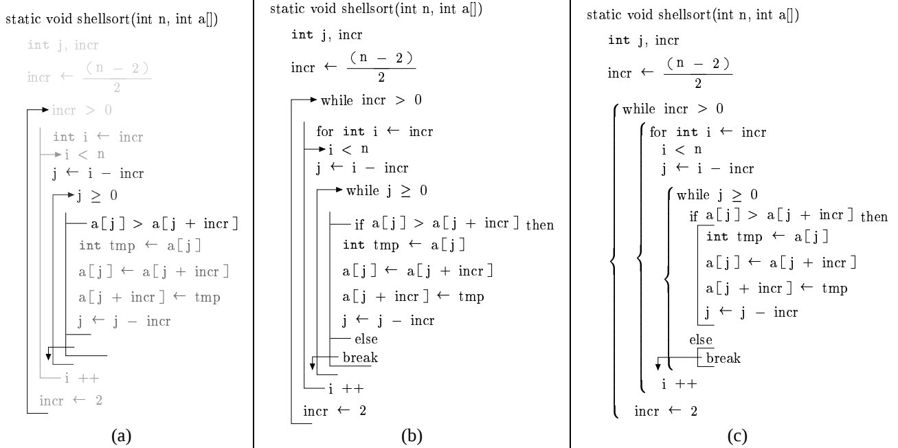
Figure 4. Three renderings of ShellSort.
