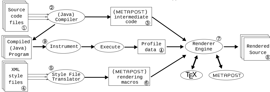
Figure 1. Overview of \mathcal{A}\mathcal{R}\mathcal{T} .
