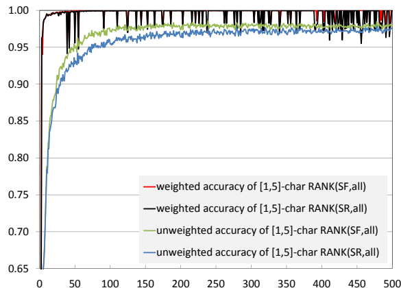
Fig. 2. Accuracy as a function of test document size in characters.
