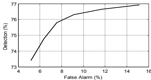
Fig. 4. The ROC curve for the detection rate and false alarm by changing the weight of garbage model.
