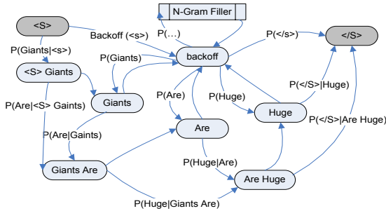
Fig. 2. Interpolated N-gram Model for a short sentence (“Giants are huge”). Transitions without labels are back-off transitions.
