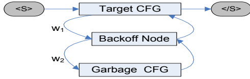
Fig. 1. An schematic illustration for proposed interpolated LM.
